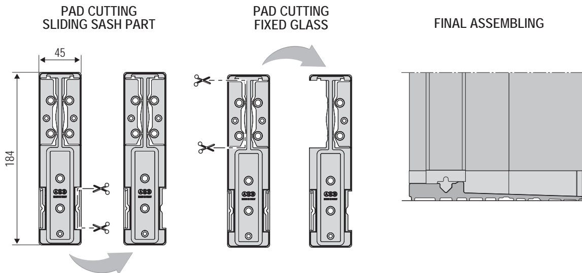
APPLICATION FOR FRAME COMPENSATING PAD (example of the left Lift&Slide)
