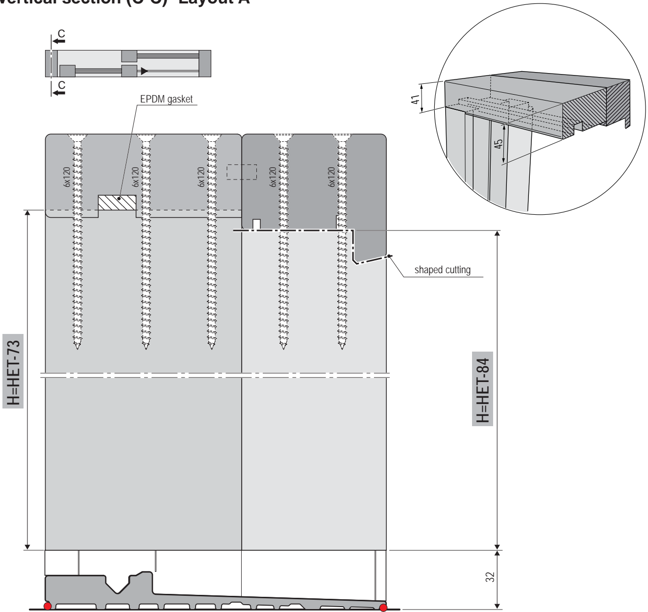
APPLICATION FOR FRAME COMPENSATING PAD (example of the left Lift&Slide)
